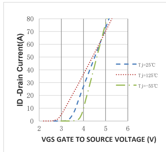
Figure 10. Transfer Characteristics
